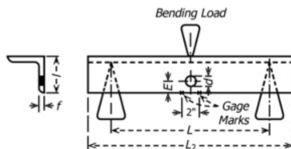
FIG. 1 Specimen for Elongation after Fracture
